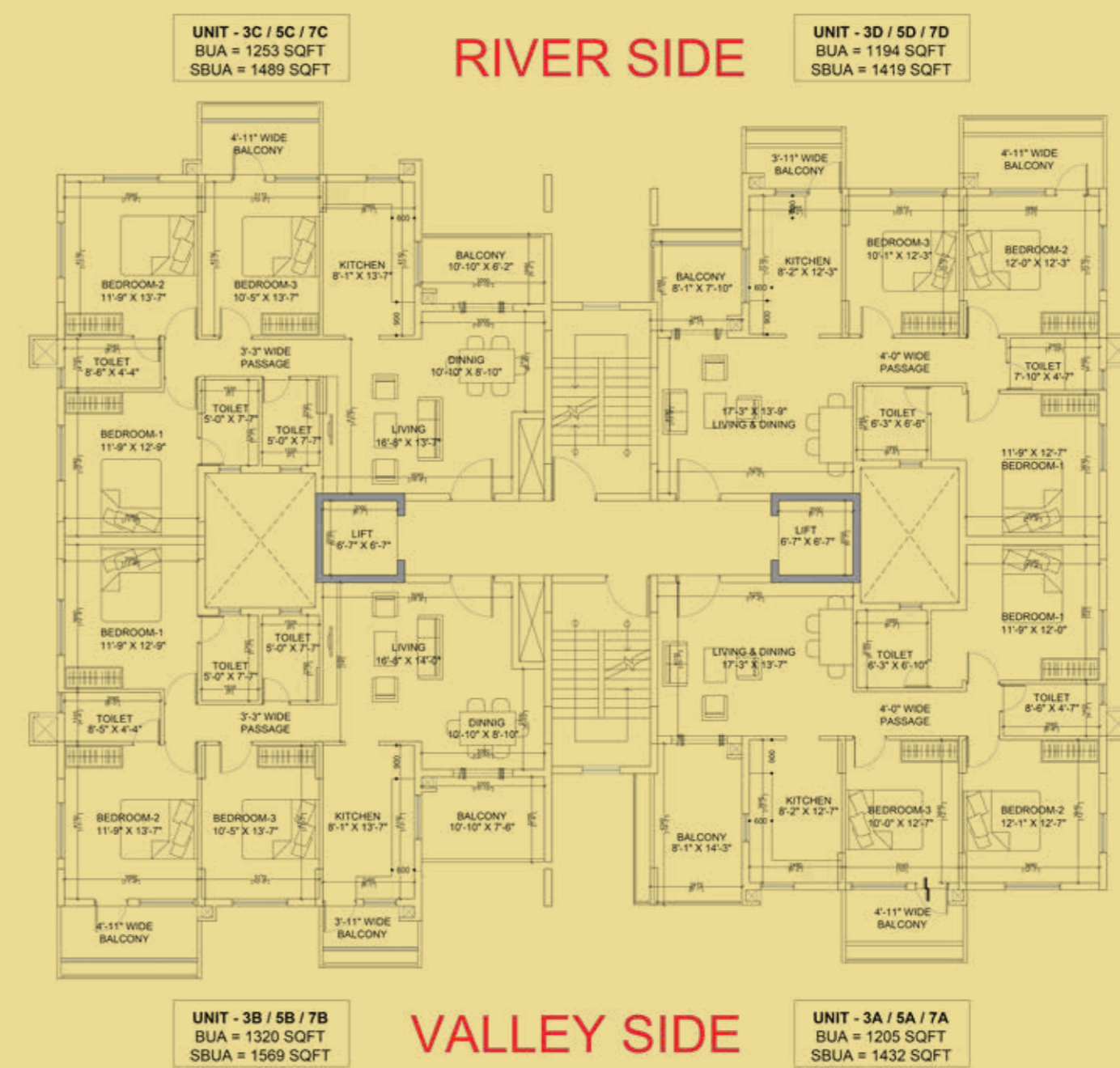
TYPE - 4 3RD , 5TH & 7TH FLOOR PLAN
