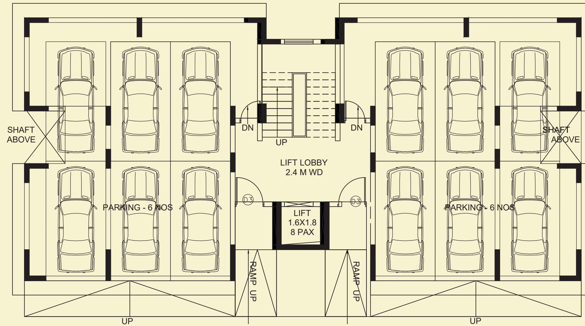
BLOCK 6 GROUND FLOOR PLAN
