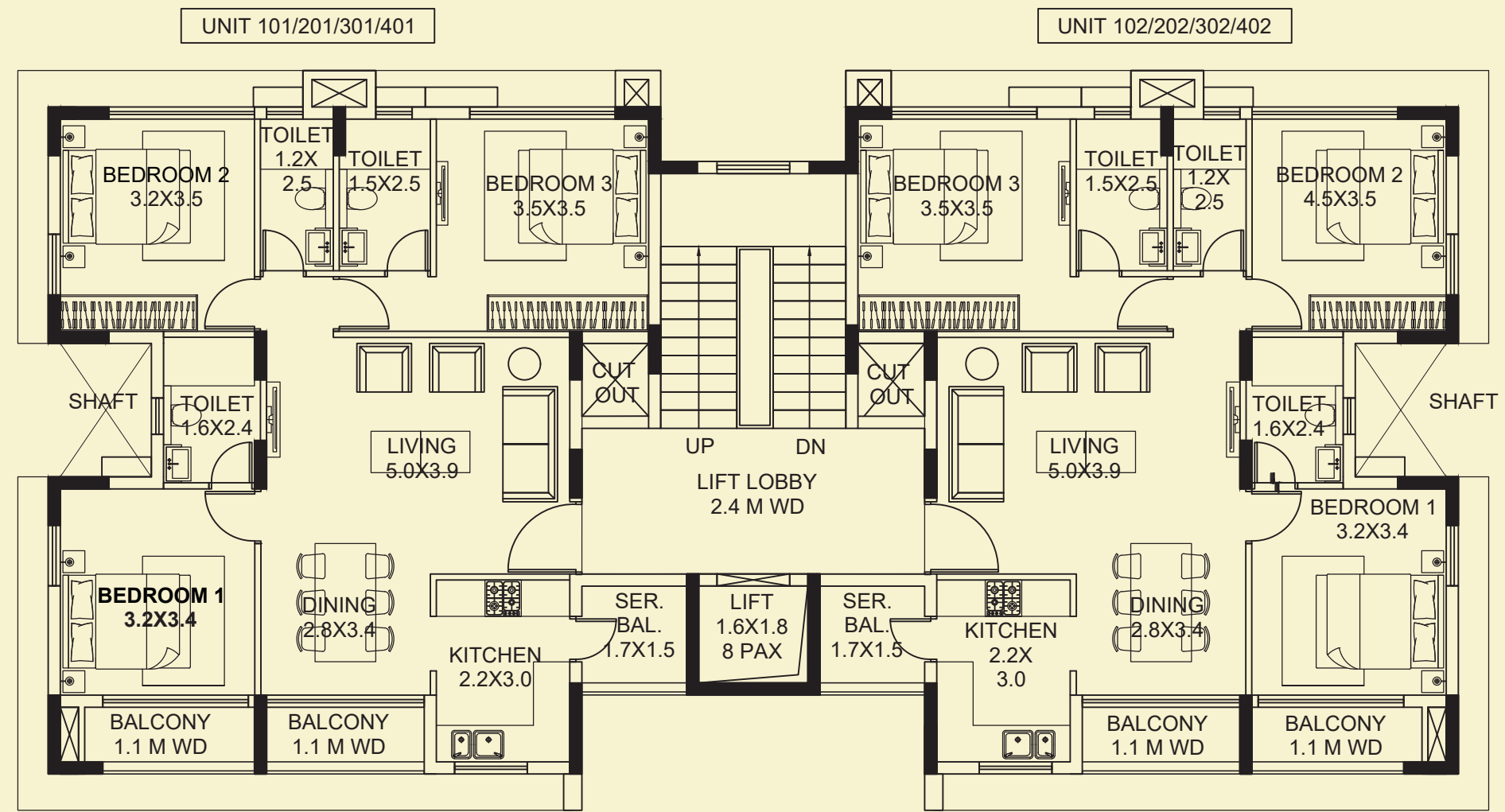
BLOCK 6 TYPICAL FLOOR PLAN
