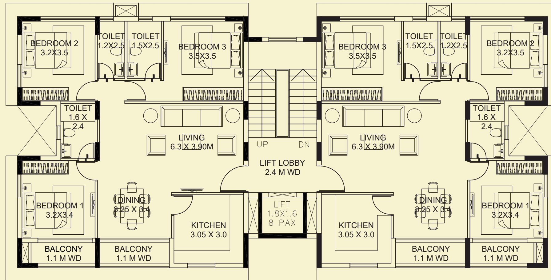
TYPICAL FLOOR PLAN
