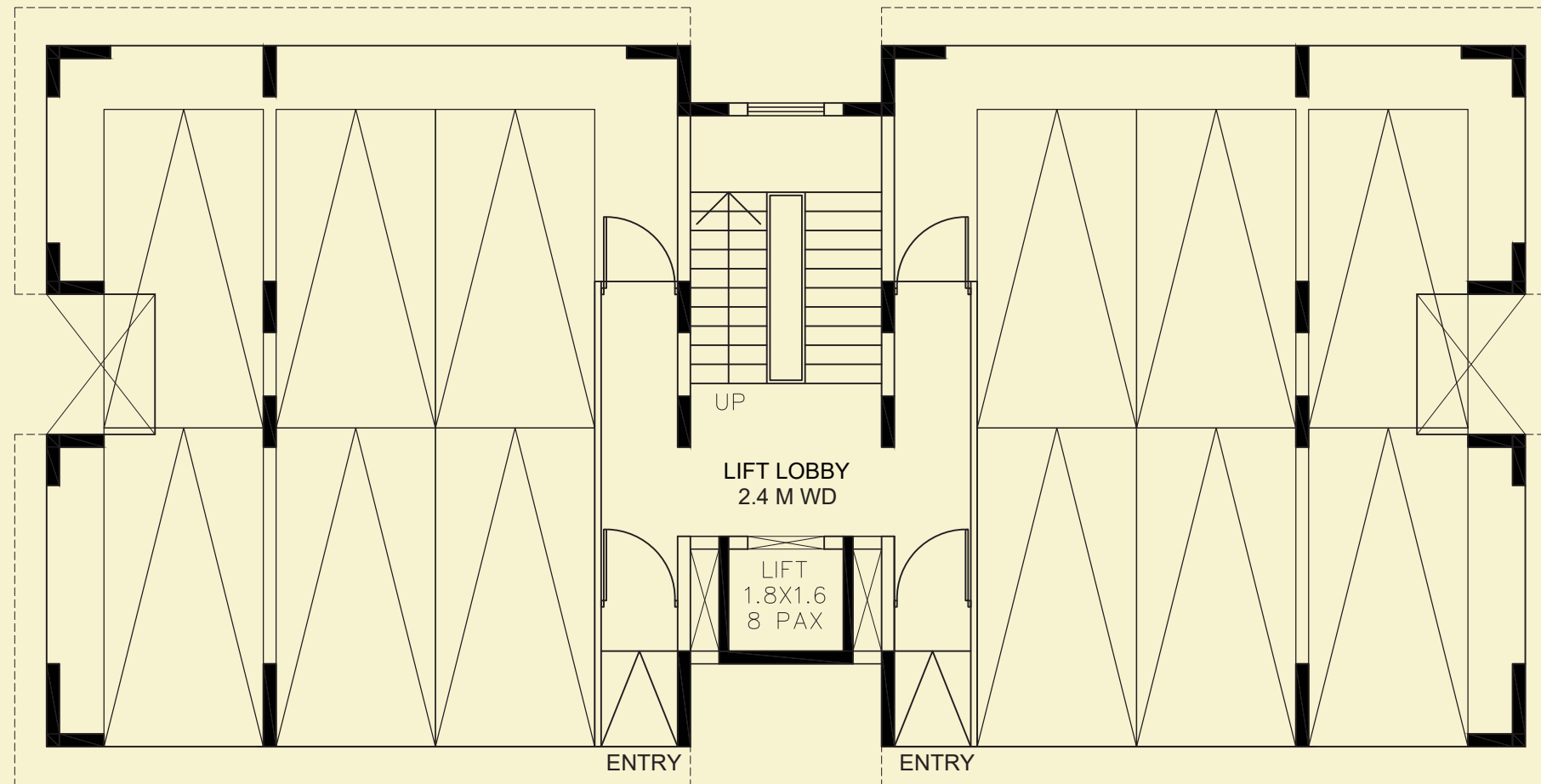
GROUND FLOOR PLAN CAR PARKING
